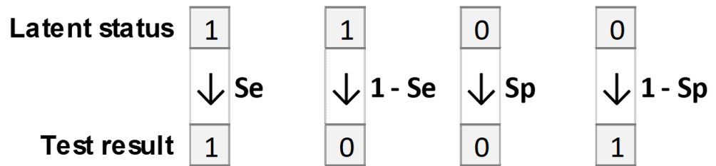
Figure 3. Relation of the model latent status to test result. Sensitivity is the probability of a positive test result in a status positive herd. Specificity is the probability of a negative test result in a status negative herd.
